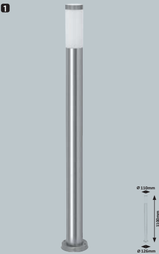
1 8265 M P E-27 / 1x max. 25W IP44 • • 9437 stainless steel/white
