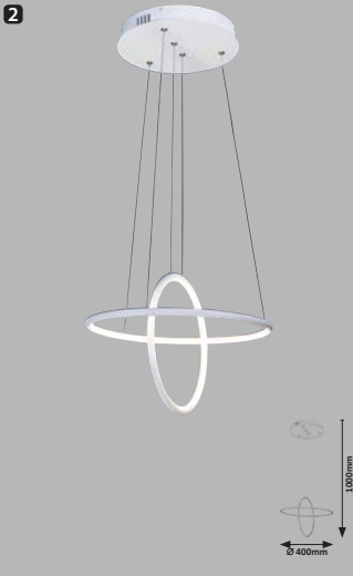
2 2544 M P • LED / 37W (2300lm, 4000K) incl. IP20 white
