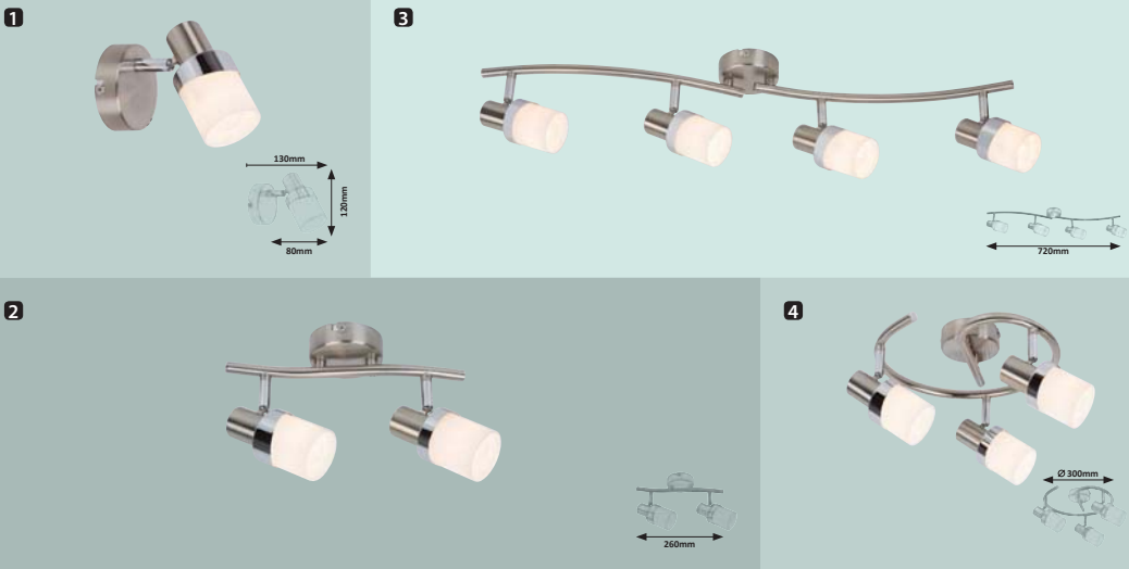
1 5631 MG E-14 / 1x max. 40W IP20 • 19633 satin chrome/ chrome/ opal glass
